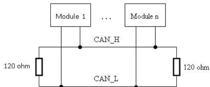
Figure 5: Bus topology
